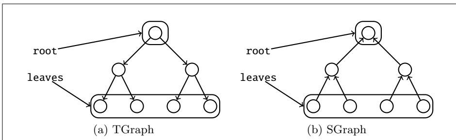
Fig. 5: MRSC data structures
